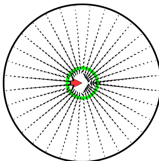
FIG. 3. (Color online) Mean displacement field after averaging over \mathcal{O}(10^5) individual fields induced by imposing a displacement dipole at the origin. The orientation of the dipole is given by the arrow. As explained in the text, the mean dipole moment vanishes after averaging and the resulting field is quadrupole. A circle at a radius \lambda=0.191L from the origin is also shown.
