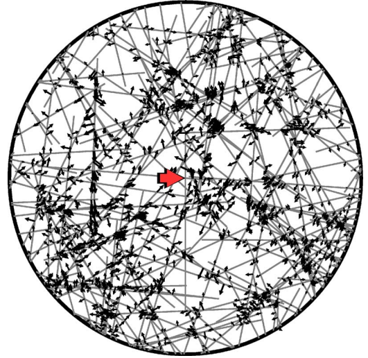
FIG. 1. (Color online) An example of a network of filaments of uniform length L (grey line segments) perturbed by an external force, denoted by the large arrow, applied to the cross link at the origin of a circular system of radius R=L . The arrow lengths are logarithmically calibrated to the magnitude of the displacement of at each cross link. In this example, L/l_c \approx 29.1 , \lambda/L \approx 0.191 , and the force is perpendicular to one of the filaments that form the central cross link; forces can also be applied parallel to a filament.
