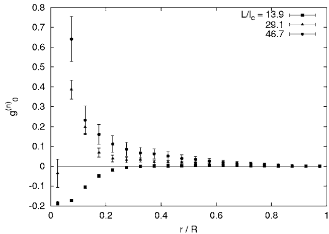
FIG. 5. g_0^{(n)} vs r/R for \lambda/L \approx 0.191 , R=L , and the L/l_c given in the key.
