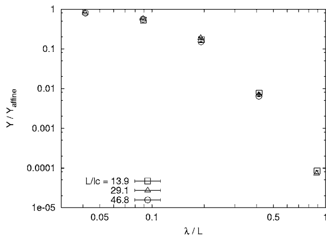
FIG. 17. Young's moduli scaled by the affine prediction vs \lambda/L on log-log axes. The affine prediction, which depends only on L/l_c , can be found in Ref. [8]. The symbols are larger than the error bars.
