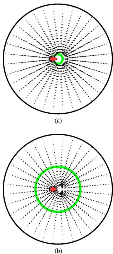
FIG. 2. (Color online) Mean response after averaging \mathcal{O}(10^5) networks with the same parameters as in Fig. 1 (including one filament fixed perpendicular to the external force) except for \lambda , which is (a) \lambda/L \approx 0.089 and (b) \lambda/L \approx 0.42 . For easy visualization, a circle of radius \lambda has been inserted into the background of each plot. Vectors near the center of each system have not been plotted for clarity.
