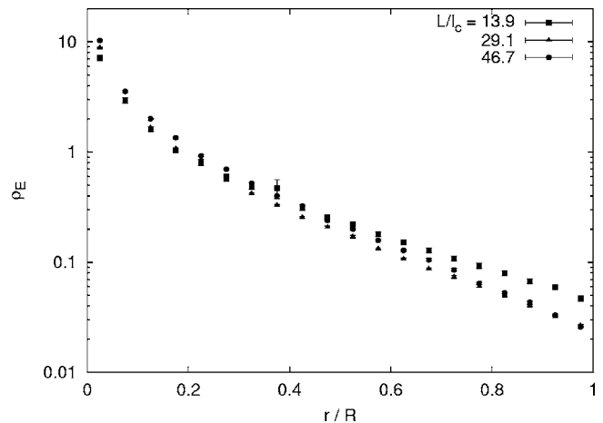
FIG. 10. Density of elastic energy \rho_E (in arbitrary units) vs distance r from an externally applied force that is directed along the filament to which it is applied. L/l_c is varied as given in the key, and R=L and \lambda/L \approx 0.191 in all cases.
