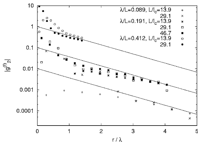
FIG. 6. Log linear plots of g_2^{(f)} vs the scaled distance from perturbation r/\lambda for systems with various values of \lambda as given in the key. The system radius R=L in all cases. Data within a boundary layer of width \lambda from r=R is not shown (see text for details).
