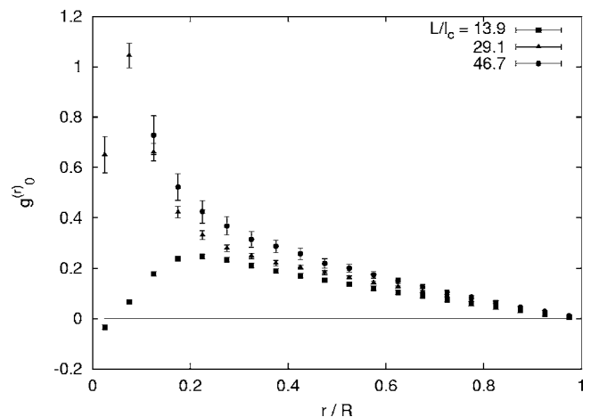
FIG. 7. g_0^{(r)} vs r/R for \lambda/L \approx 0.191 , R=L , and differing L/l_c as shown in the legend.
