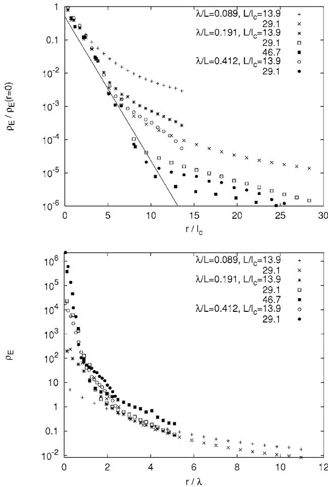
FIG. 11. Scaled elastic energy density vs distance from the point force for a variety of networks—see legend. In each case the force is directed perpendicularly to the filament where it is applied. In the upper panel distances are scaled by l_c and the data have been collapsed in the small r/l_c regime. The solid line is proportional to \exp(-r/l_c) , showing l_c controls the initial decay of elastic energy. In the lower panel the same energy densities are plotted against distance scaled by \lambda . This shows the energy density decays with that characteristic length scale at longer ranges. Error bars are not shown for reasons of clarity.
