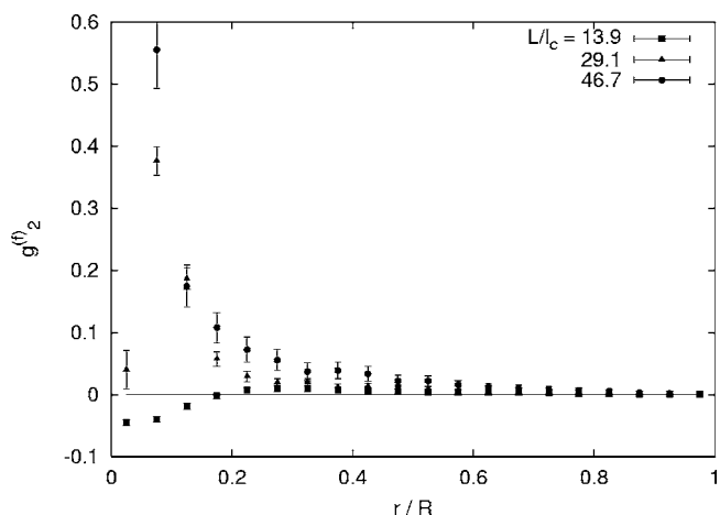
FIG. 4. g_2^{(f)} (which is dimensionless) vs distance from point of force application r for systems with the same \lambda/L \approx 0.191 and cross-link densities L/l_c as given in the key ( L is the filament length). The system radius R=L in all cases.
