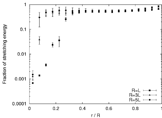
FIG. 14. The fraction of elastic energy stored in the \mathcal{H}^{\parallel} term of the Hamiltonian for perpendicular forces, as a function of distance from the origin r for system sizes R=L , 3L , and 5L . In all cases L/l_c \approx 29.1 and \lambda \approx 0.191L .
