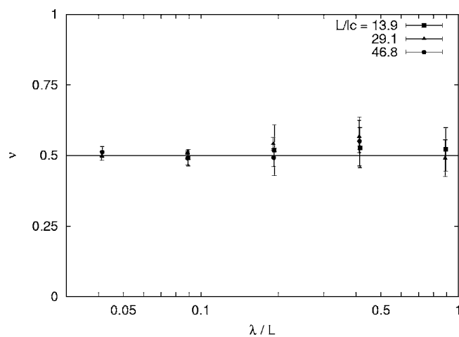
FIG. 18. The Poisson ratio \nu for the same systems as in Fig. 17. The solid line corresponds to \nu = \frac{1}{2} .
