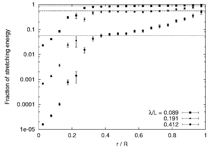
FIG. 13. The fraction of elastic energy due to filament stretching in networks with the same L/l_c \approx 29.1 (in fact, the exact same geometries), R=L but different \lambda . The different values of the stretching energy fraction in the intermediate regime reflect the differing values of the ratio L/\lambda for the networks. For comparison, the macroscopic energy fraction under bulk shear is shown as horizontal dashed lines, in the same order as the data points (i.e., \lambda/L \approx 0.089, 0.191, \text{ and } 0.412 from top to bottom).
