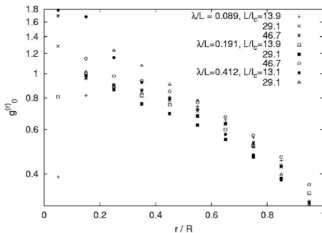
FIG. 9. g_0^{(r)} vs r/R for R=3L on log-linear axes, with \lambda/L and L/l_c as given in the key. Each curve has been shifted vertically by a \lambda -dependent scale factor to attempt data collapse. Since \lambda varies by over a factor of 4, the rough collapse is enough to rule out any significant \lambda dependence on the decay. Error bars are not shown for clarity.
