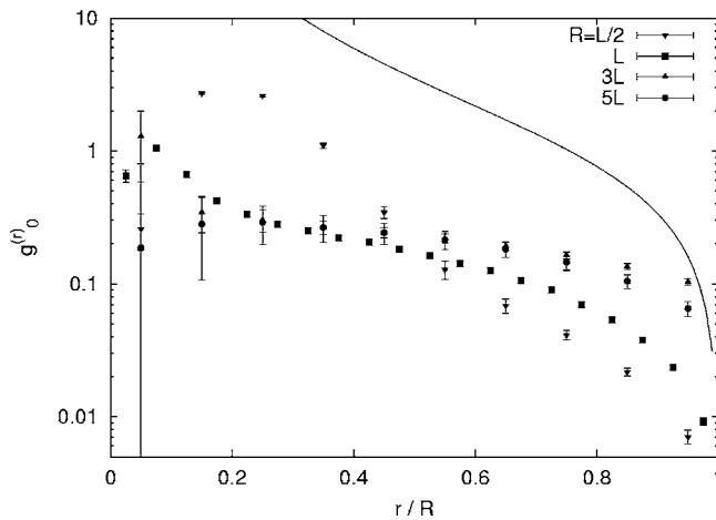
FIG. 8. g_0^{(r)} vs r/R for \lambda/L \approx 0.191 , L/l_c \approx 29.1 , and the system radii R given in the key. The continuum response for the bulk elastic moduli corresponding to these parameter values [as given by Eq. (A3)] is shown as a solid line.
